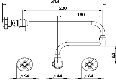
Easy Clean Wall Stops & Outlet
