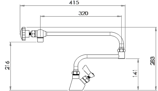
Stainless Single Deck Tap Outlet only
